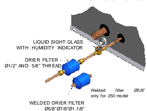
MOUNTING DIAGRAM DRIER FILTER AND LIQUID SIGHT GLASS
