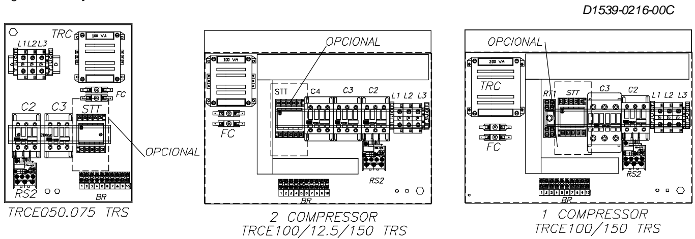
Fig. VII-55 - Layout - TRCE - Standard.
