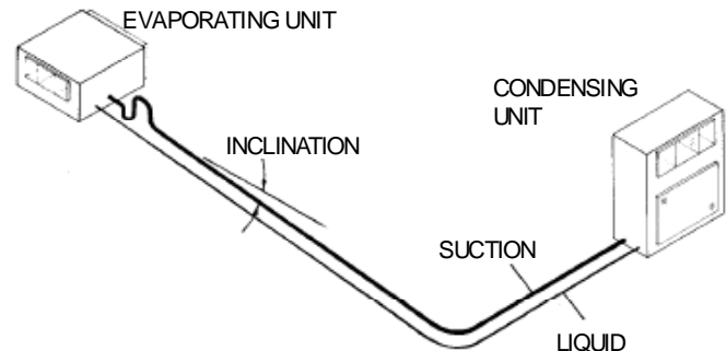
Fig.IV-03 - Assembly diagram for EU at the same level as CU
