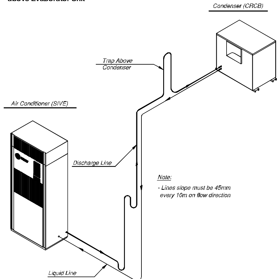
Figure IV-06 - Recommendations For Refrigerating Installation. Condenser Unit above Evaporator Unit
