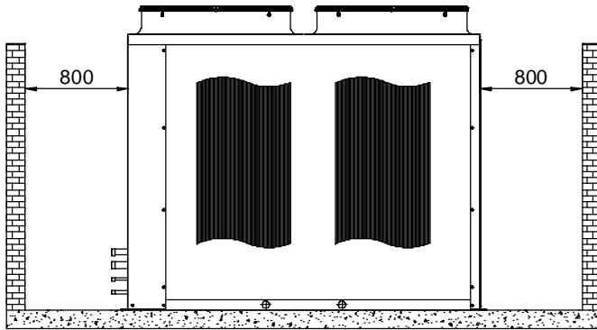
Fig. VIII-18 - Suggested Clearances for Maintenance and Air Circulation - Condensing Unit TRCE 050 to 150.
