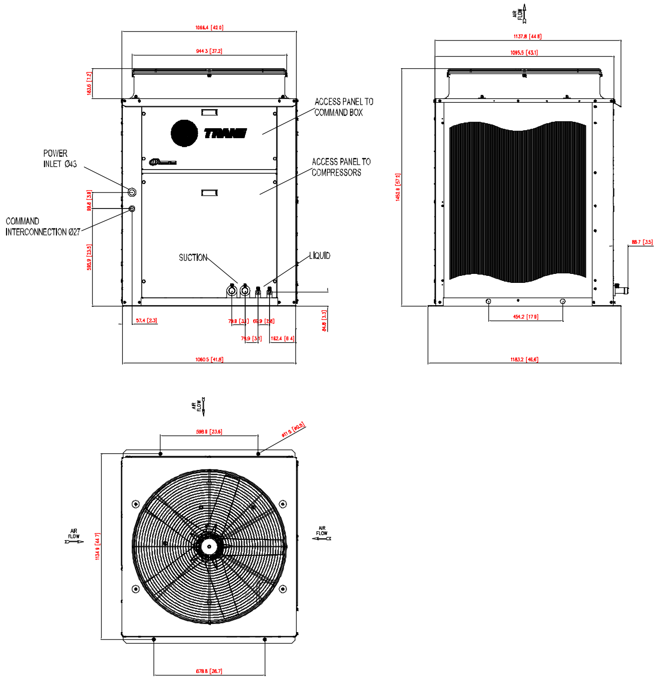
Fig. VIII-12 - Dimensions - Condensing Units TRAE 250 - 2 Circuits
