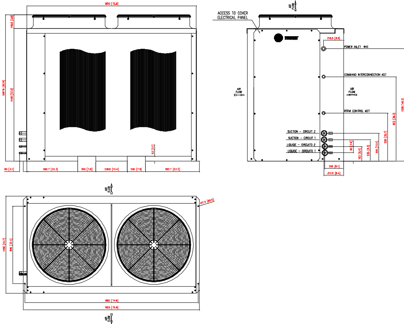
Fig. VIII-13 - Dimensions - Condensing Units TRAE 300 - 2 Circuits
