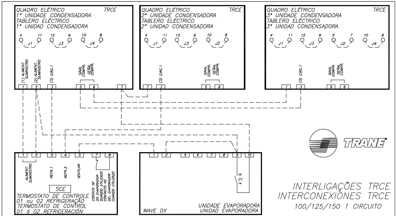
Fig. VII-59 - Wiring Diagram Evaporator Unit + Condensing Unit (TRCE)
