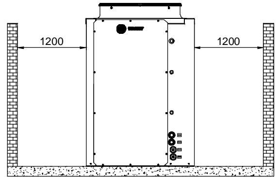
Fig. VIII-18 - Suggested Clearances for Maintenance and Air Circulation - Condensing Unit TRCE 050 to 150.
