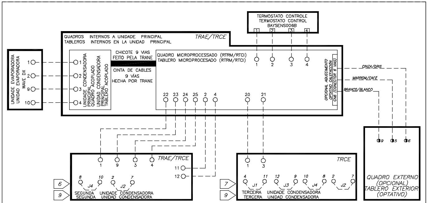
Fig. VII-59 - Wiring Diagram Evaporator Unit + Condensing Unit (TRCE)
