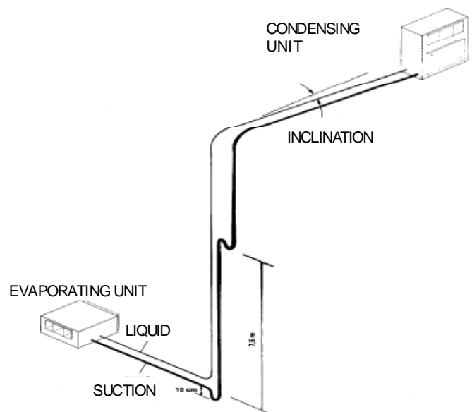
Fig. IV-02 - Assembly Condensing Unit over Evaporating Unit.
