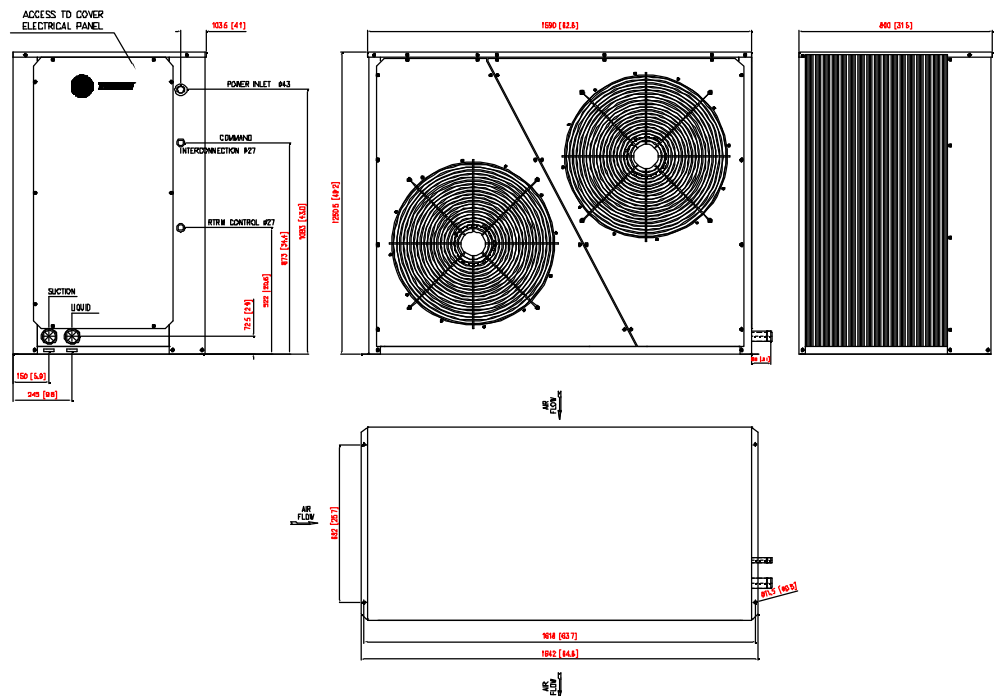
Fig. VIII-06 - Dimensions - Condensing Units TRAE 150 - 1 circuit
