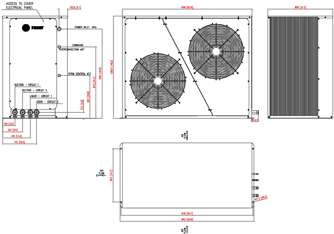
Fig. VIII-07 - Dimensions - Condensing Units TRAE 150 - 2 circuits
