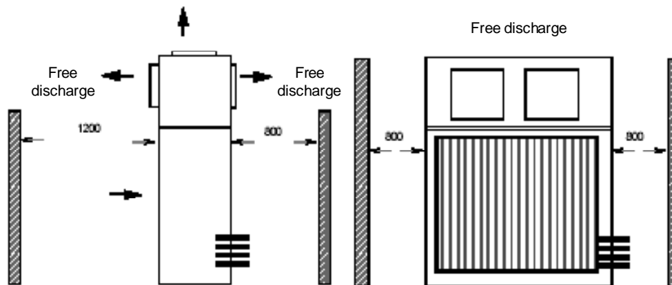
Fig. VIII-18 - Suggested Clearances for Maintenance and Air Circulation - Condensing Unit TRCE 050 to 150.
