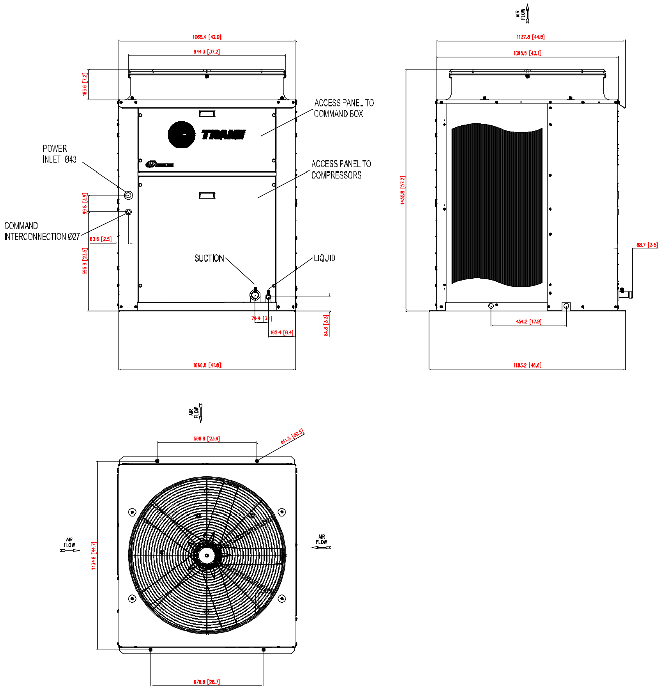
Fig. VIII-09 - Dimensions - Condensing Units TRAE 200 - 1 Circuit
