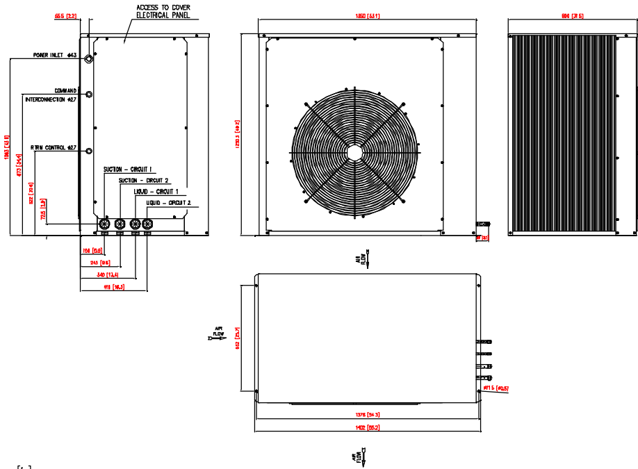
Fig. VIII-05 - Dimensions - Condensing Units TRAE 125
