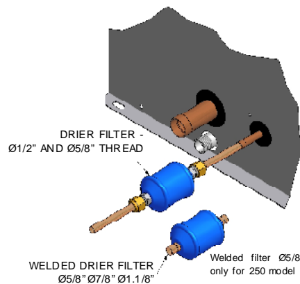
MOUNTING DIAGRAM DRIER FILTER
