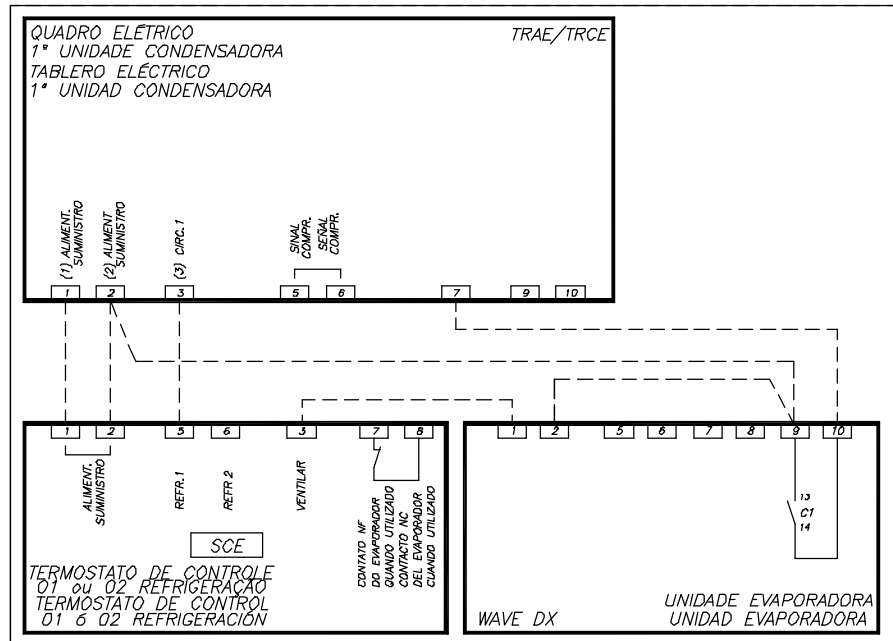
Fig. VII-57 - Wiring Diagram Evaporator Unit + Condensing Unit (TRAE/TRCE)
