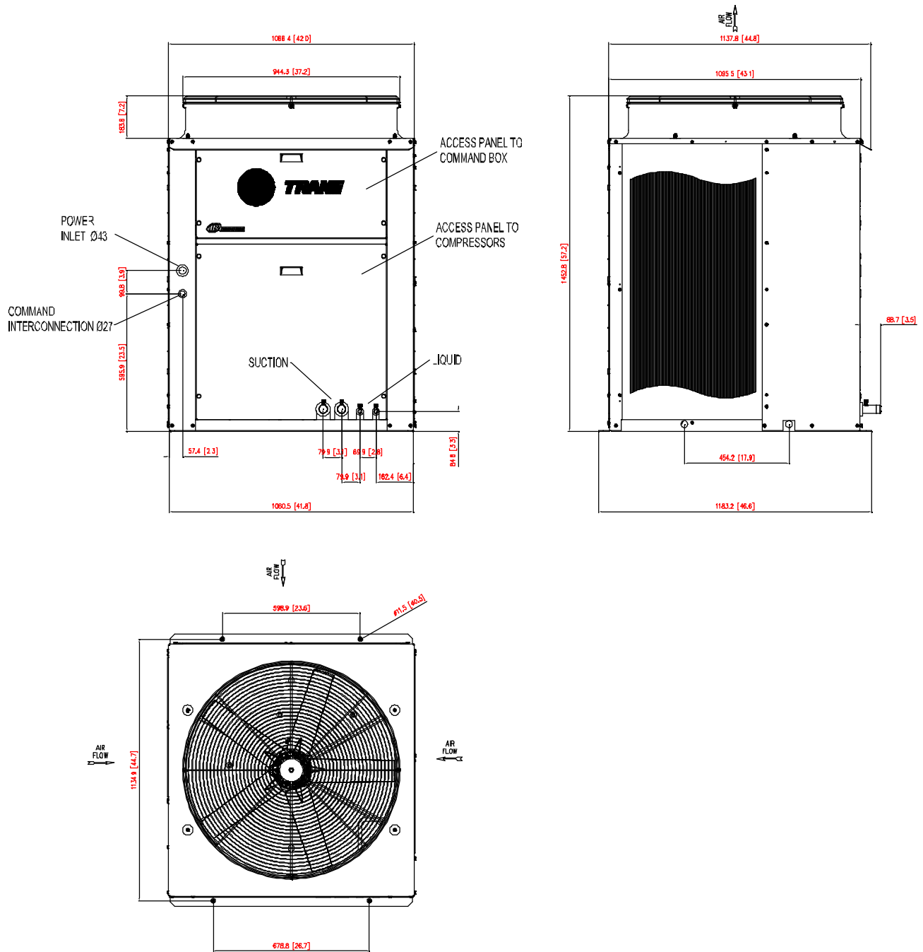
Fig. VIII-10 - Dimensions - Condensing Units TRAE 200 - 2 Circuits
