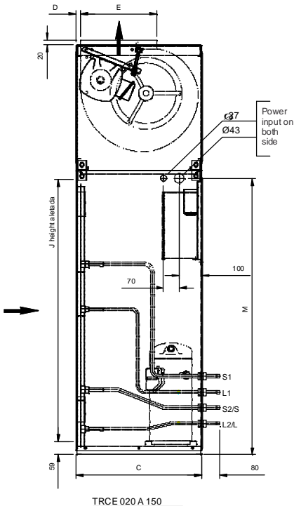
Fig. VIII-15 - Connections - condensing unit TRCE
