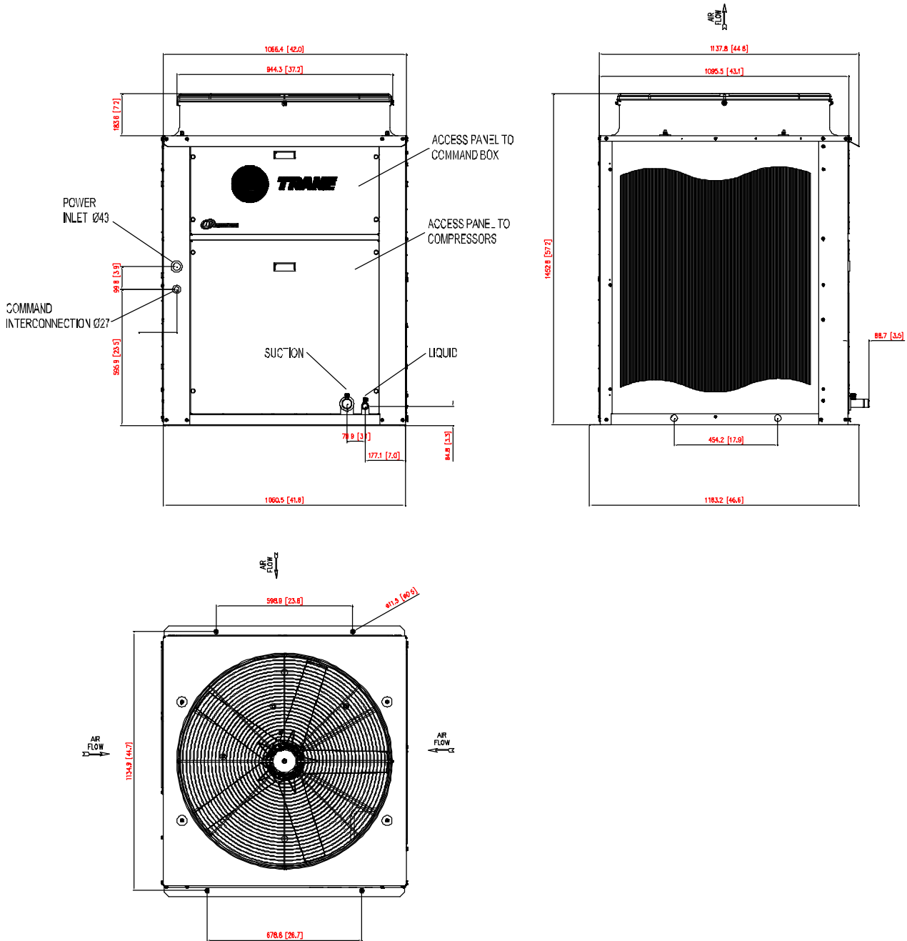
Fig. VIII-11 - Dimensions - Condensing Units TRAE 250 - 1 Circuit
